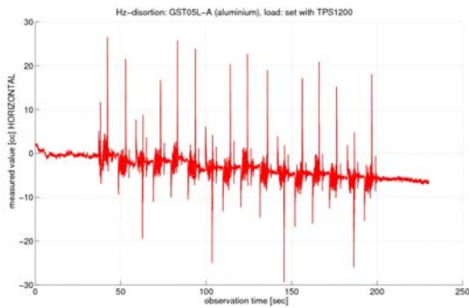
Figure 6b - Leica GST05L tripod
