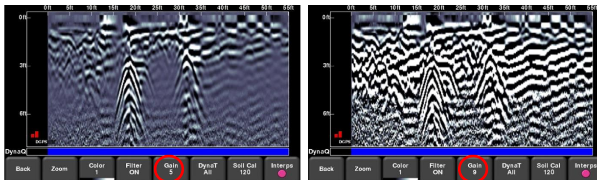
Figure 8-10: Varying the Gain
