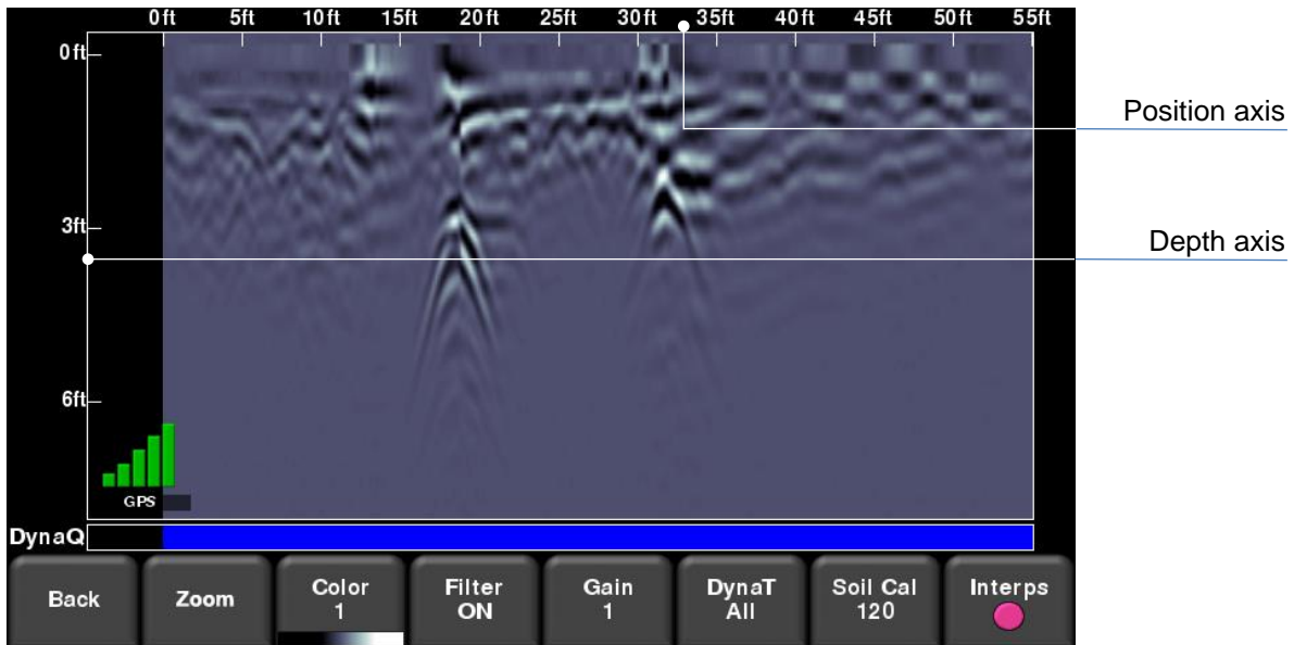
Figure 8-3: Line Scan acquisition mode, showing collected data and axis labels
