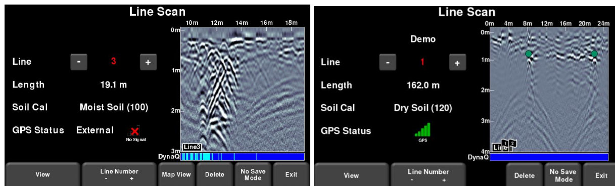
Figure 8-2: Line Scan mode, showing a line that was previously collected (a) RD1500 on left, (b) RD1500 Enhanced on right. The RD1500 has the MapView option on this screen.
