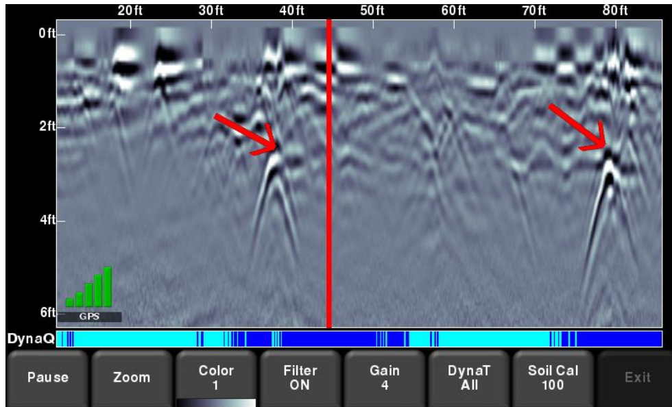
Figure 8-18: Drawing arrows on the screen to highlight targets and features
