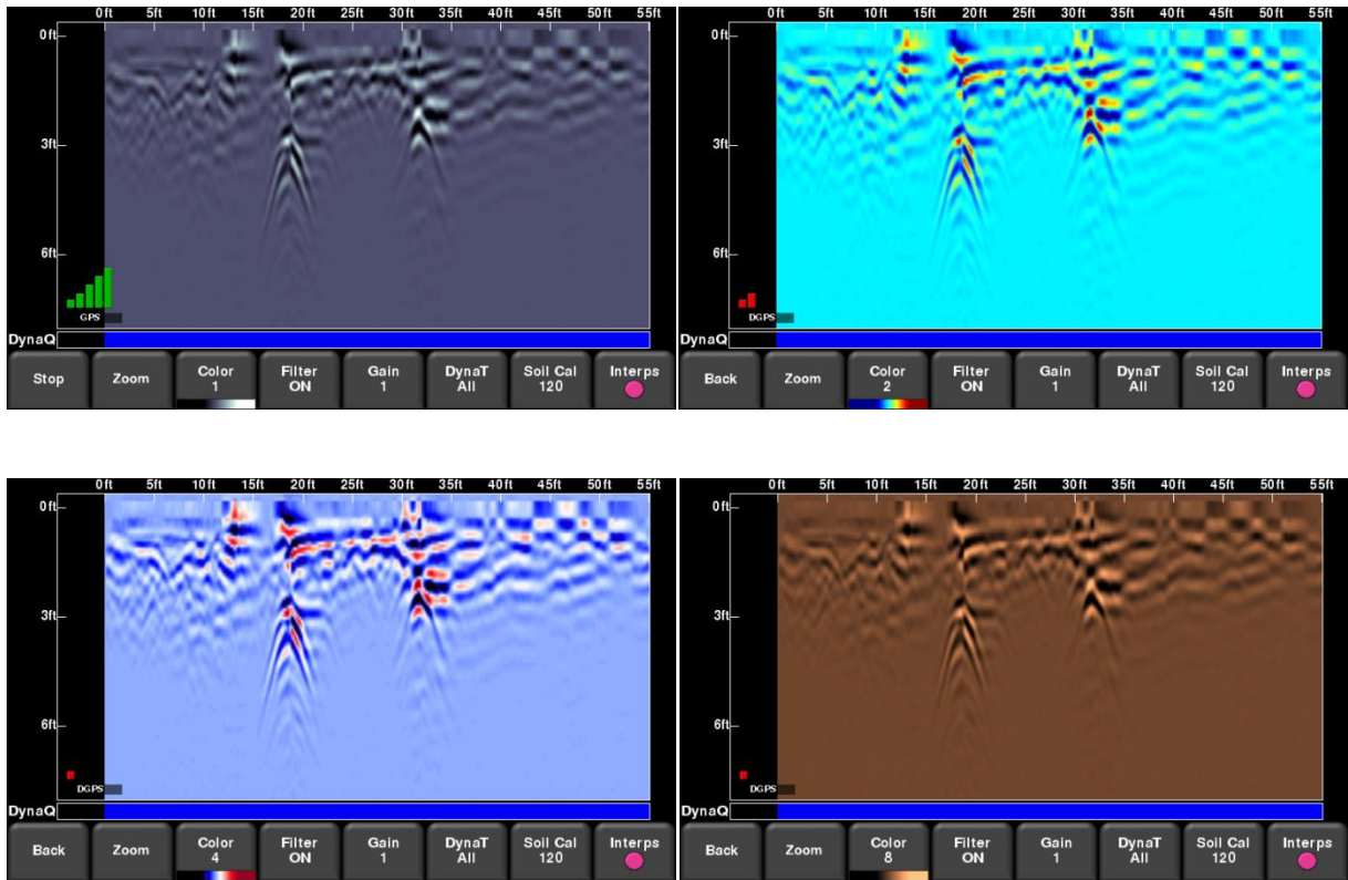
Figure 8-9: Changing Color palettes
