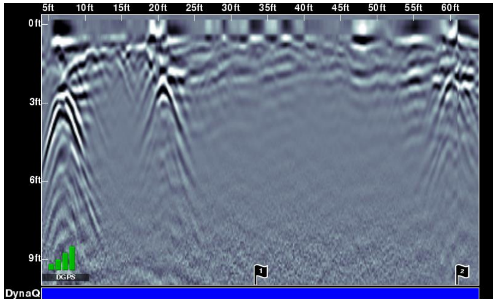
Figure 8-6: Inserting Flags
