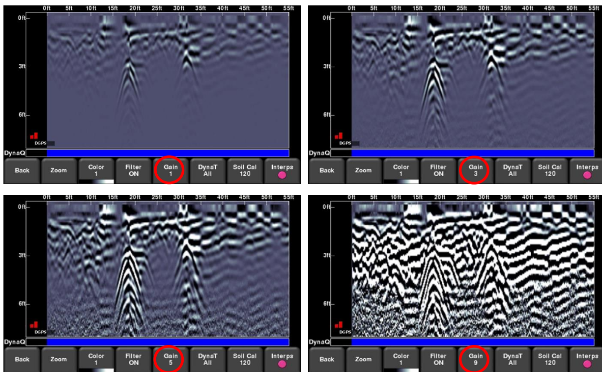
Figure 8-11: Varying the Gain
