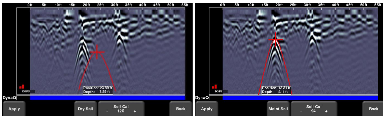
Figure 8-13: Adjusting Soil Cal, a) initial screen. b) moving the red hyperbola over a hyperbolic response from a subsurface target
