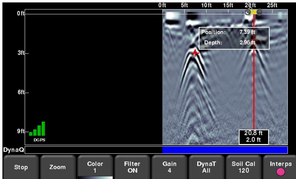
Figure 8-5: Touch screen to get depth and horizontal position at any point
