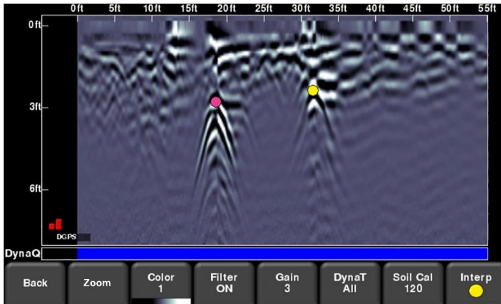
Figure 8-14: Touching the screen to add Interps
