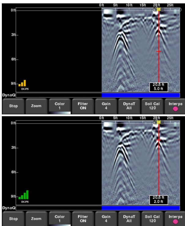
Figure 8-4: a) Back-up Indicator, b) Moving the Depth Indicator to the top of the hyperbola
