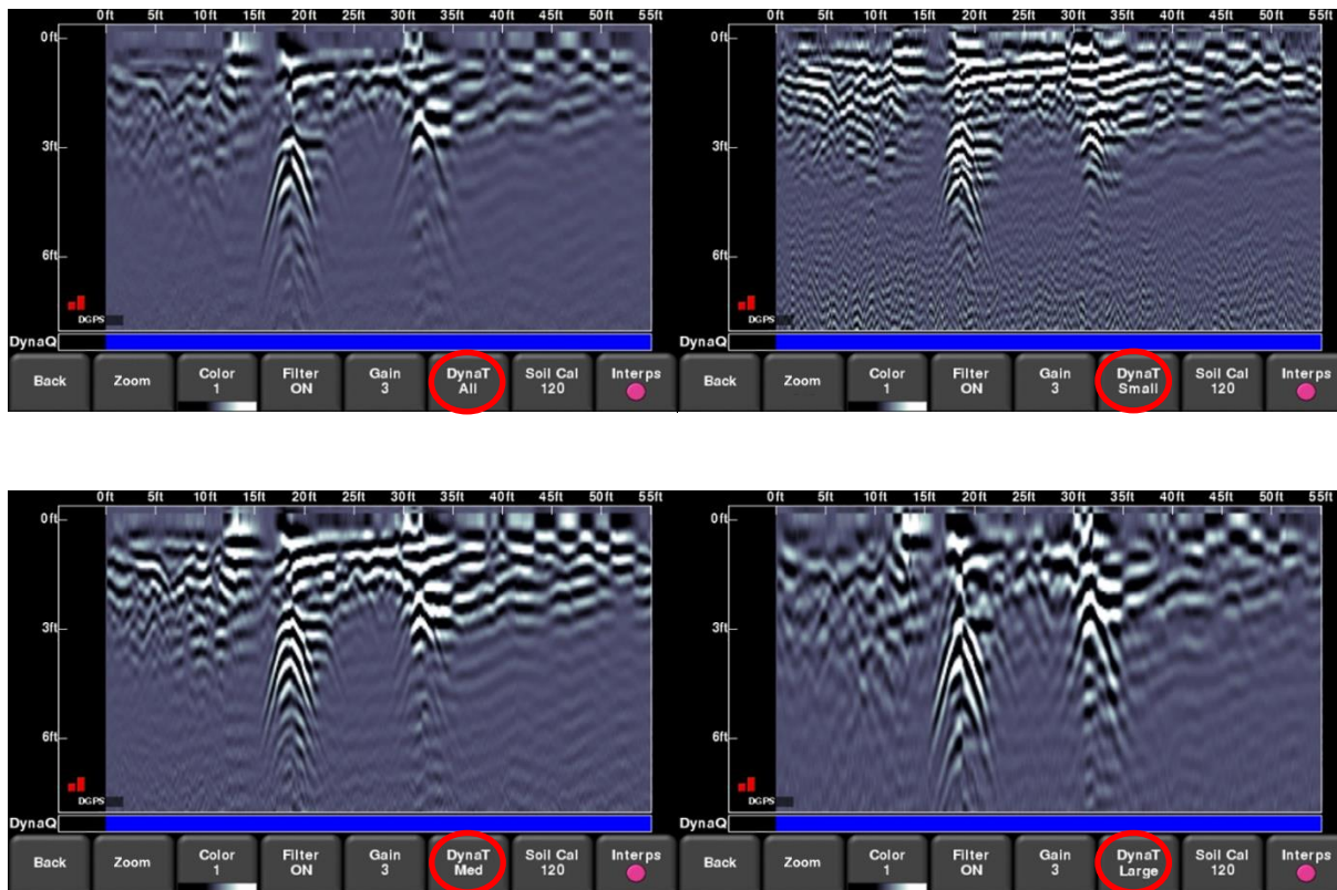
Figure 8-12: FrequenSee™ settings: a) Top left shows All . b) Top right set to Small targets. c) Bottom left set to Medium targets. d) Bottom right set to Large targets
