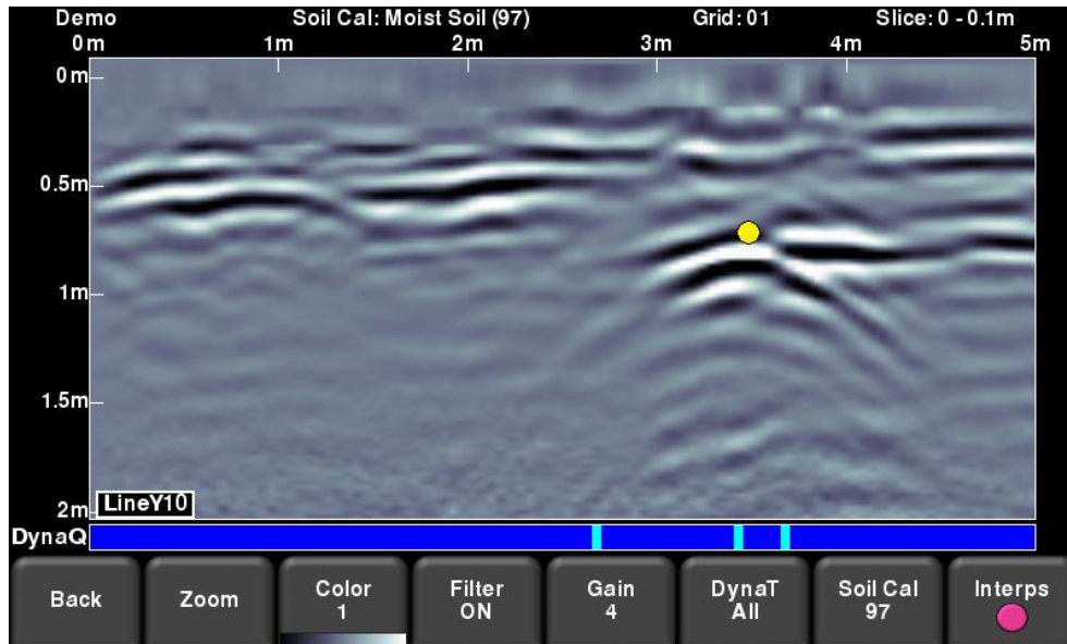
Figure 10-4: Changing Line View settings from within Slice View.
