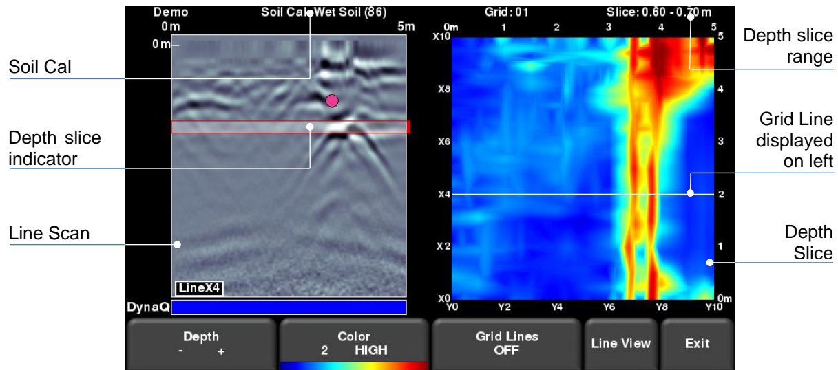
Figure 10-1: Slice View screen
